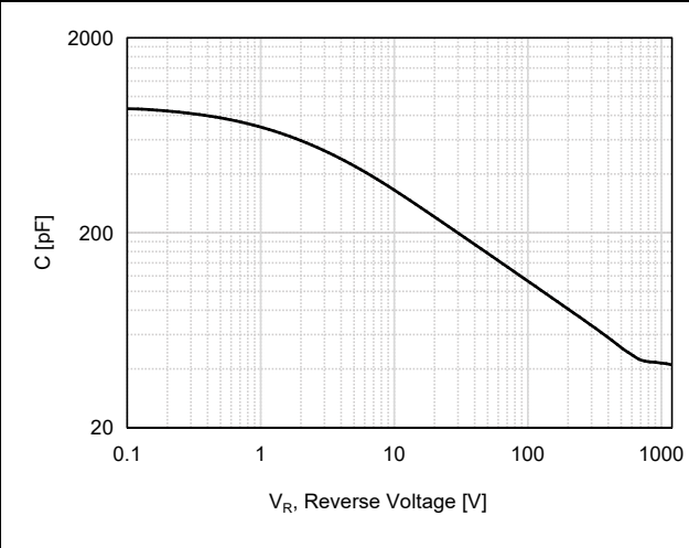
Figure 7. Capacitance Characteristic
